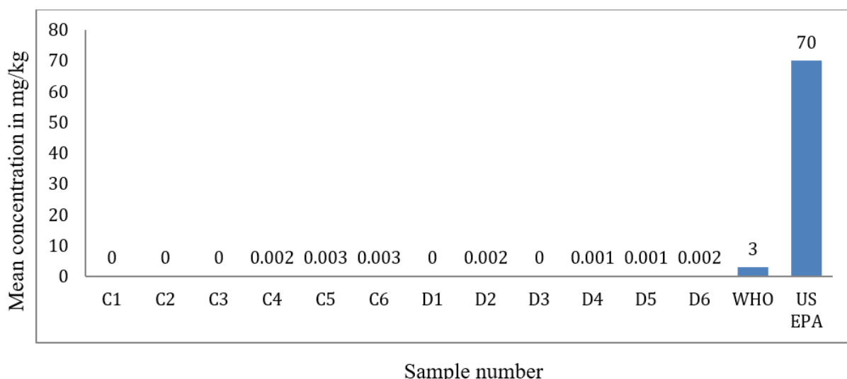
Figure 2.12: Summary of the statistical analysis of Cadmium concentration in the soil samples during dry season
