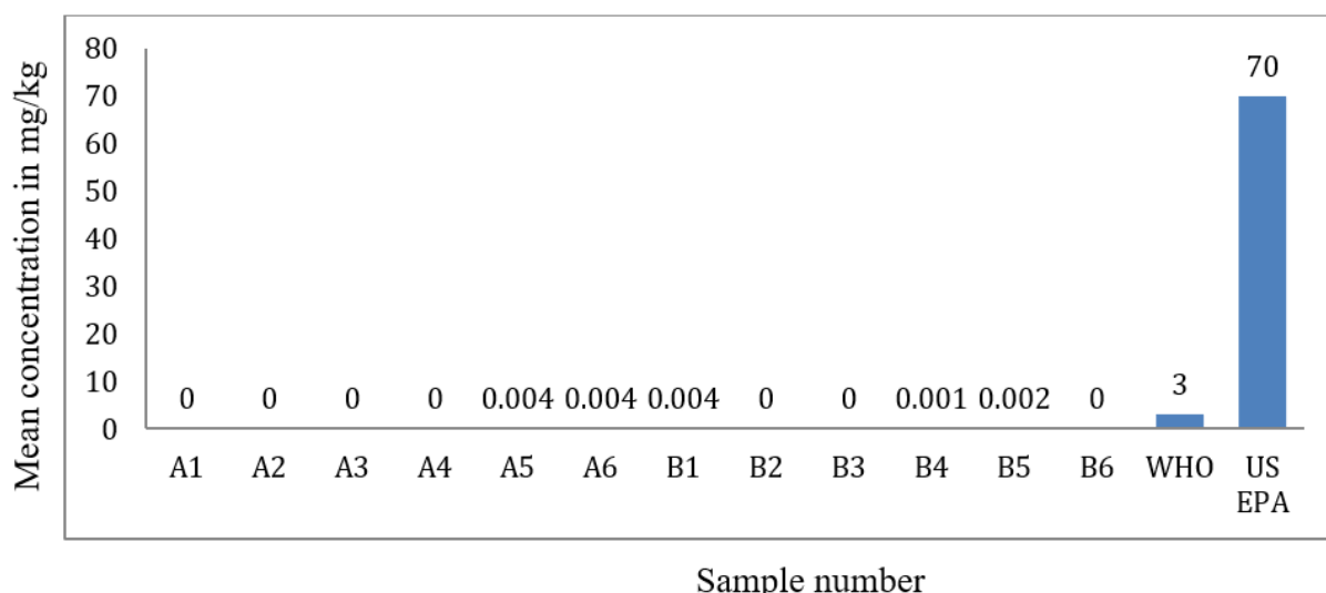
Figure 2.11: Summary of the statistical analysis of Cadmium concentration in the soil samples during dry season
