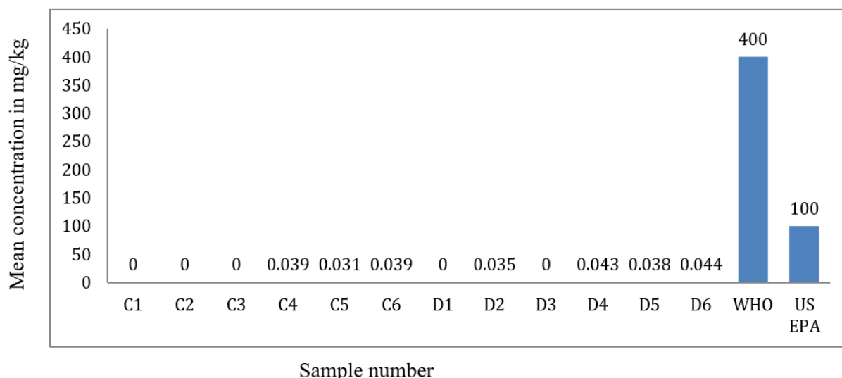
Figure 2.8: Summary of the statistical analysis of lead concentration in the soil samples during the dry season.
