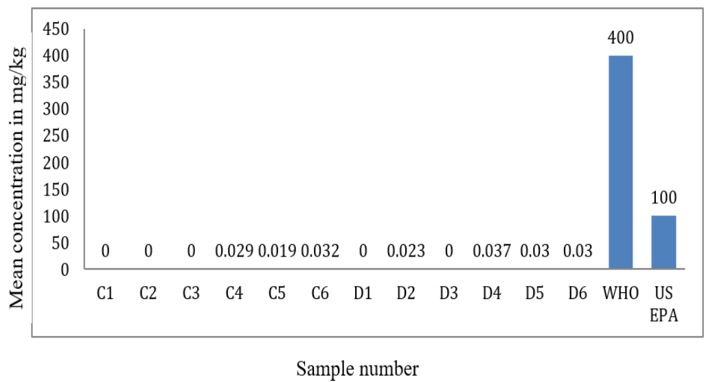
Figure 2.6: Summary of the statistical analysis of lead concentration in the soil samples during wet season
