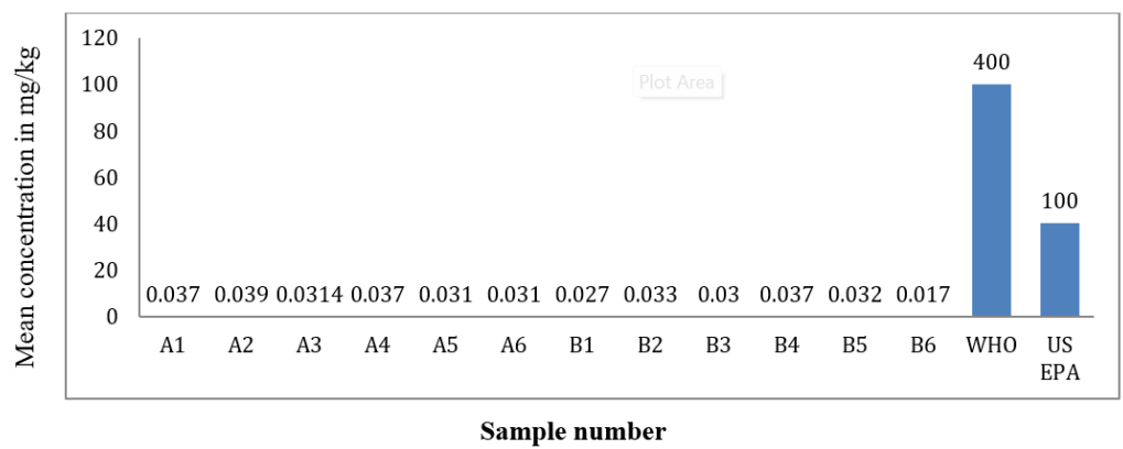
Figure 2.7: Summary of the statistical analysis of lead concentration in the soil samples during dry season
