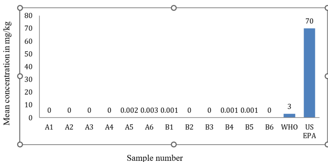
Figure 2.9: Summary of the statistical analysis of Cadmium concentration in the soil samples during wet season.
