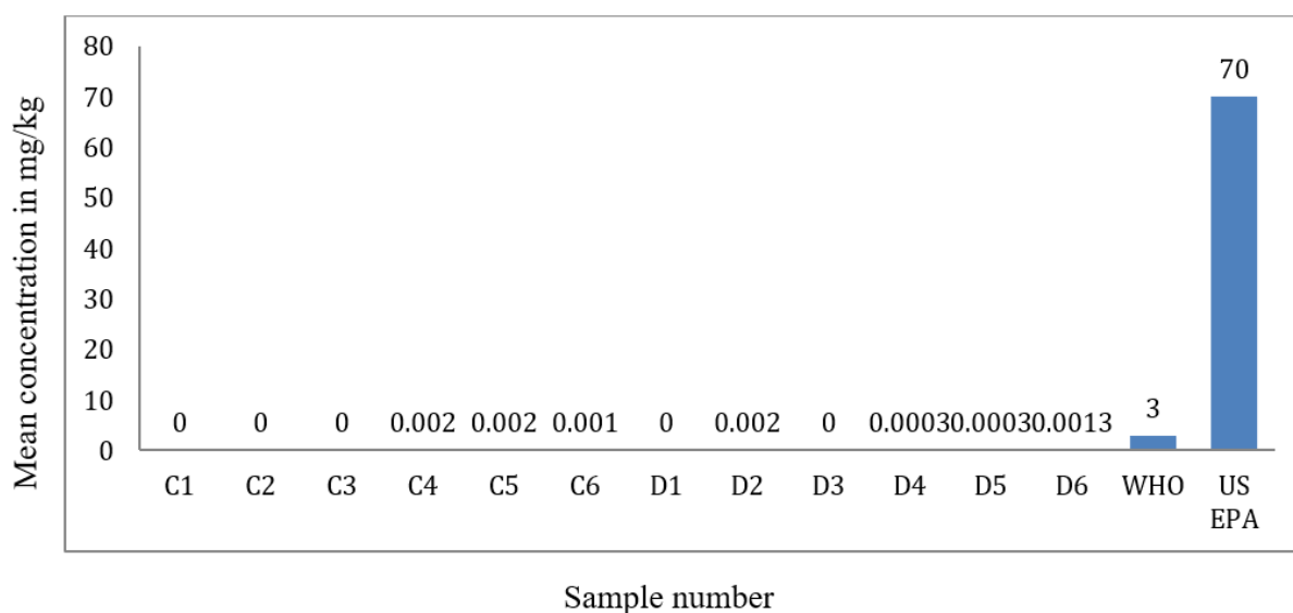
Figure 2.10: Summary of the statistical analysis of Cadmium concentration in the soil samples during wet season
