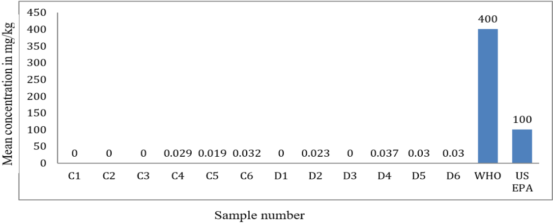
Figure 2.5: Summary of the statistical analysis of lead concentration in the soil samples during wet season
